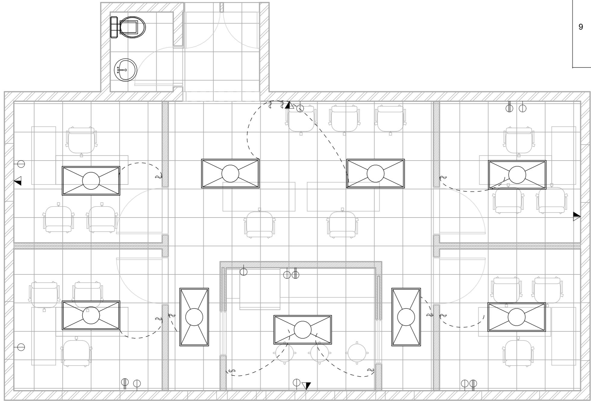
1 ELECTRICAL PLAN 1/4" = 1'-0"
