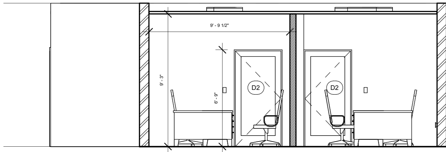
2 Section 4 1/4" = 1'-0"
