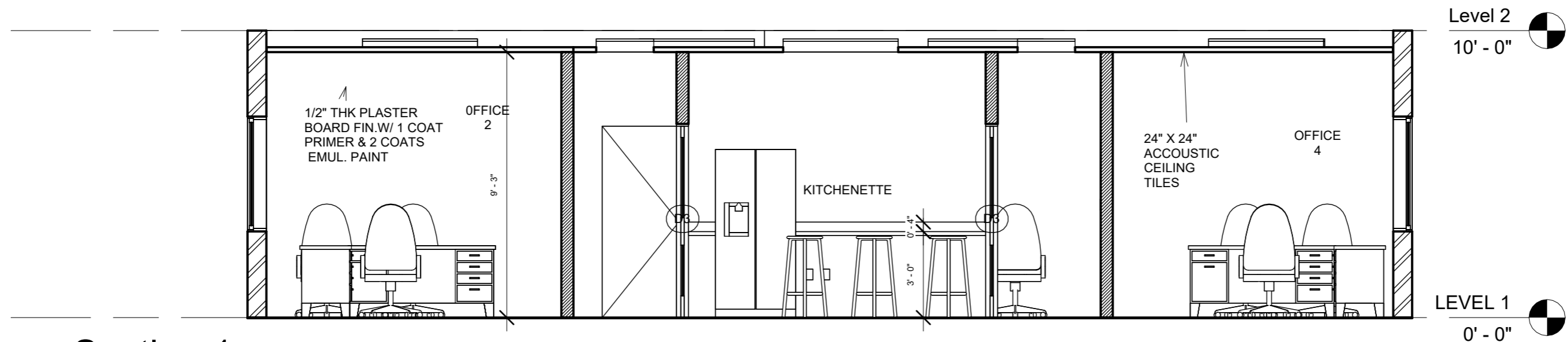
1 Section 1 1/4" = 1'-0"
