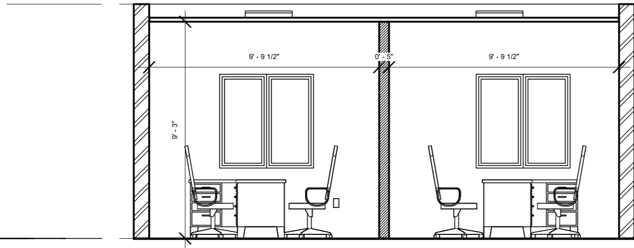
1 Section 3 1/4" = 1'-0"
