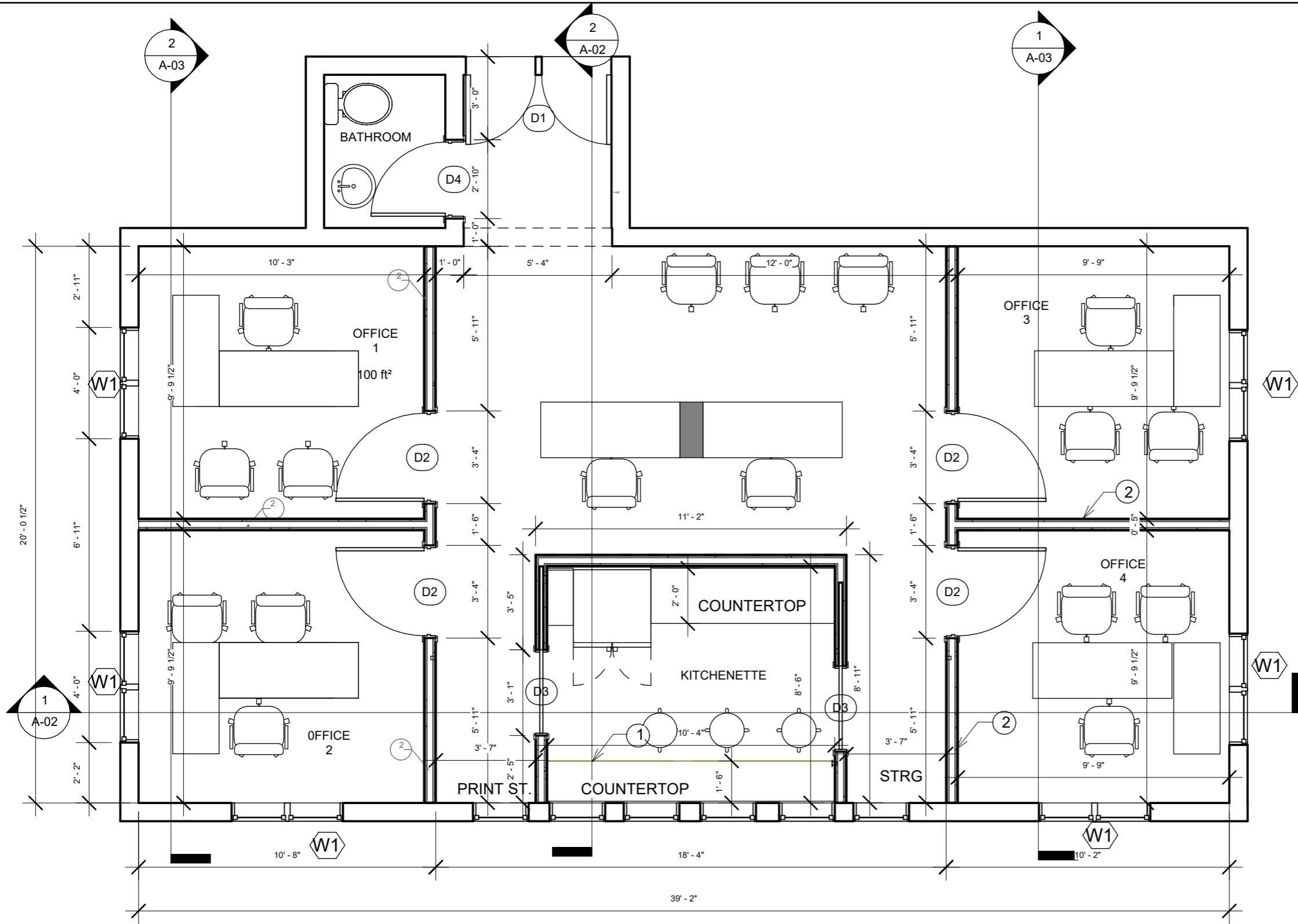
1 FLOOR PLAN 1/4" = 1'-0"
